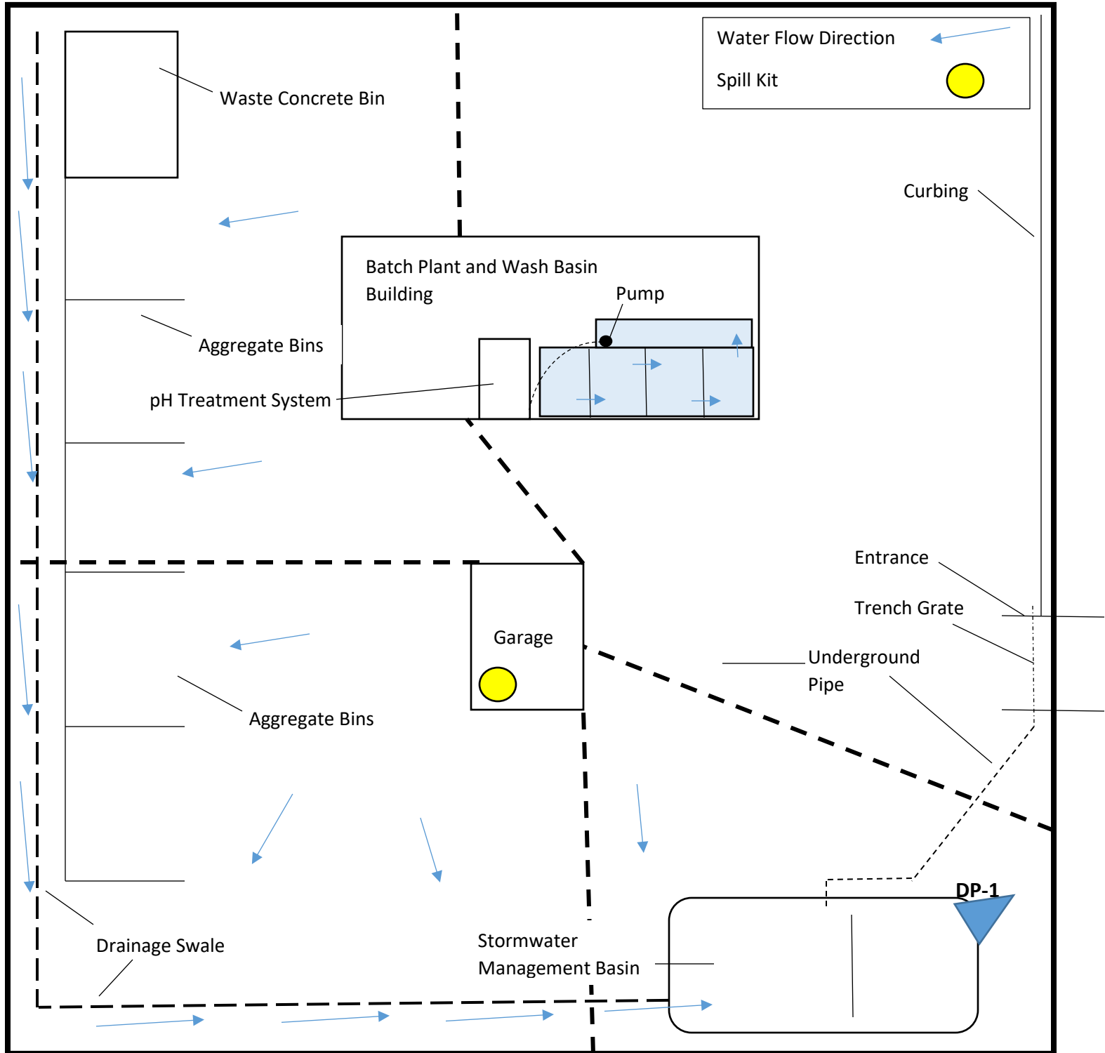
FIGURE 2 FACILITY SKETCH OF EXISTING CONDITIONS
